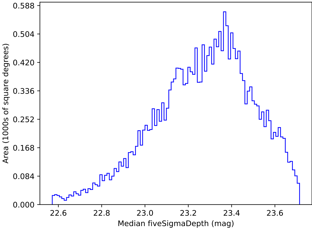
too_ignore_10_1v3.4_10yrs Yr 1 u band: Median fiveSigmaDepth
