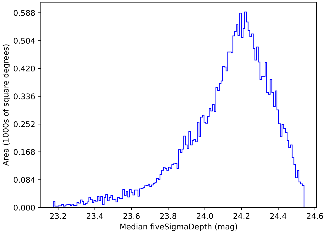
too_ignore_10_1v3.4_10yrs Yr 1 r band: Median fiveSigmaDepth
