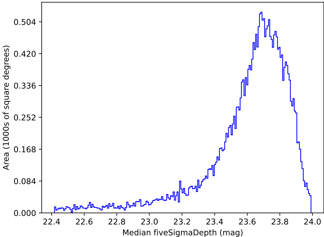
too_ignore_10_1v3.4_10yrs Yr 1 i band: Median fiveSigmaDepth
