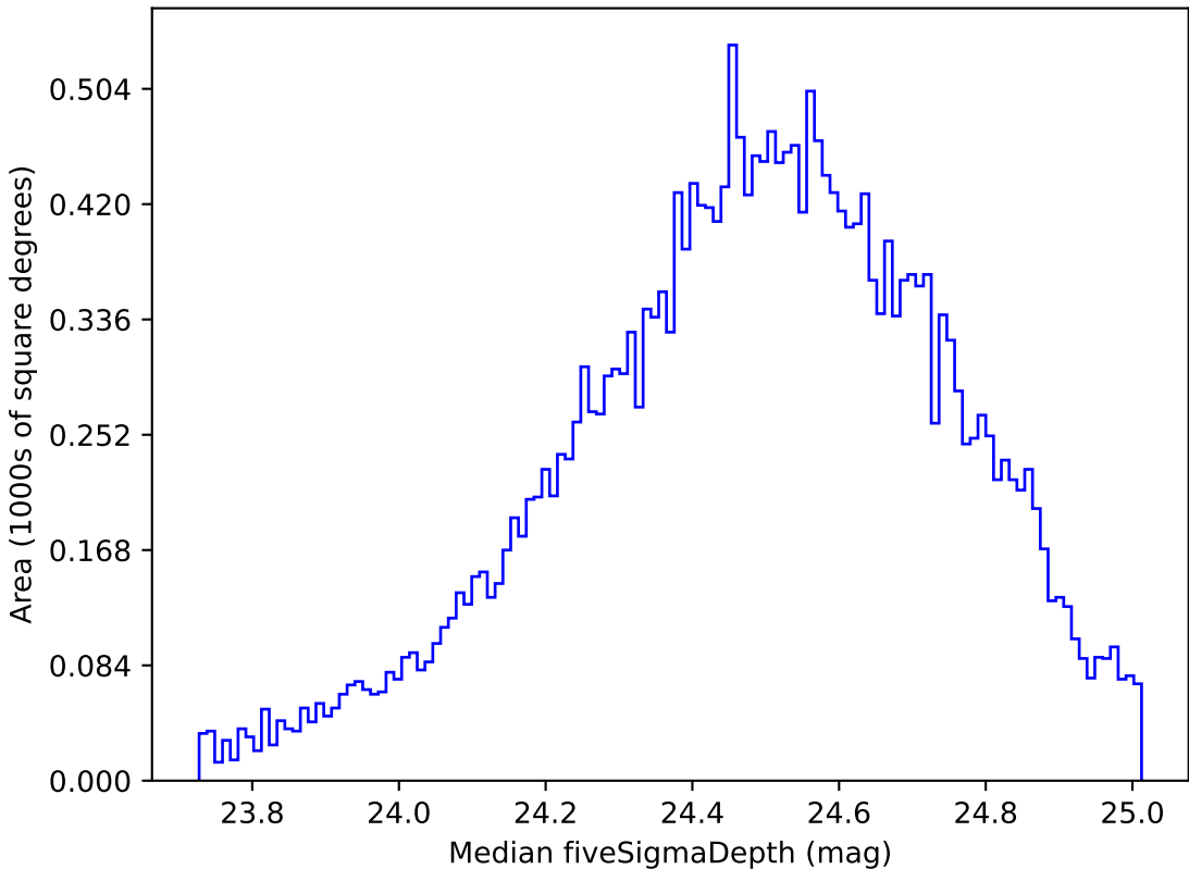
too_ignore_10_1v3.4_10yrs Yr 1 g band: Median fiveSigmaDepth
