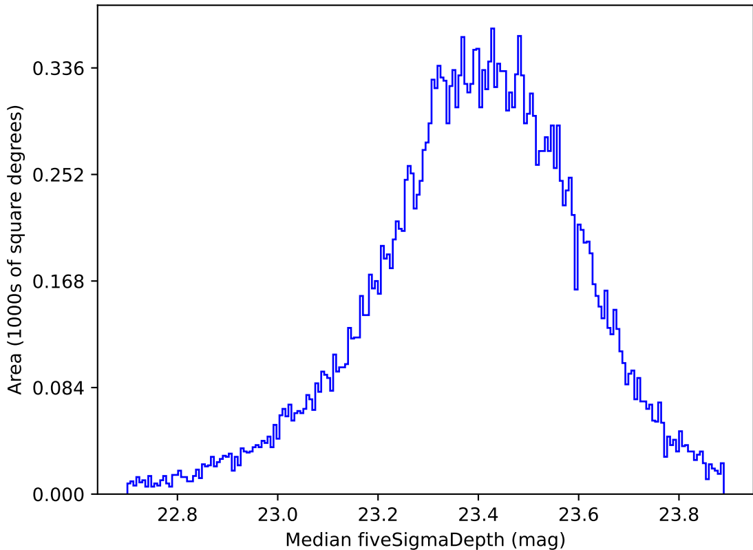
too_ignore_10_1v3.4_10yrs Yr 1 all bands: Median fiveSigmaDepth
