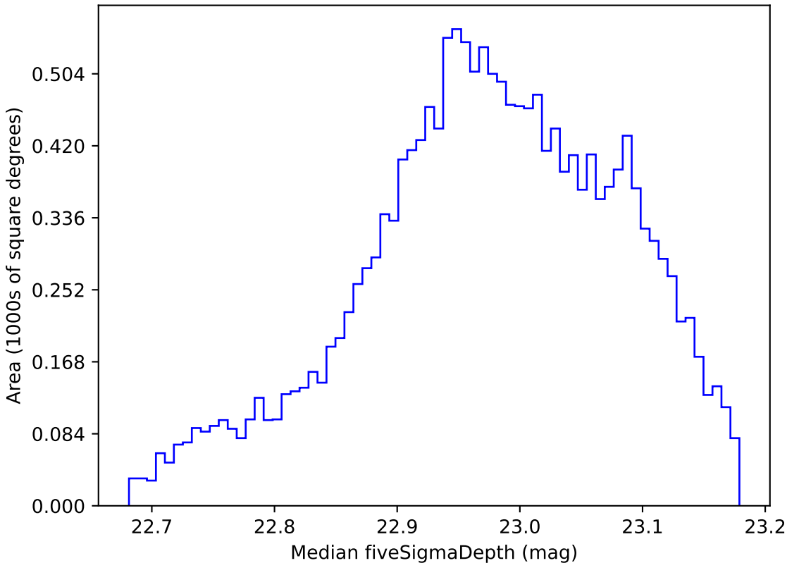
too_ignore_10_1v3.4_10yrs WFD z band: Median fiveSigmaDepth
