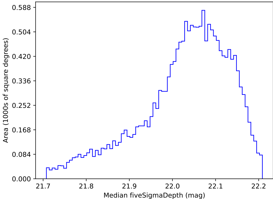
too_ignore_10_1v3.4_10yrs WFD y band: Median fiveSigmaDepth
