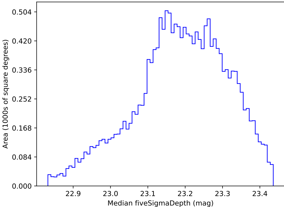
too_ignore_10_1v3.4_10yrs WFD u band: Median fiveSigmaDepth
