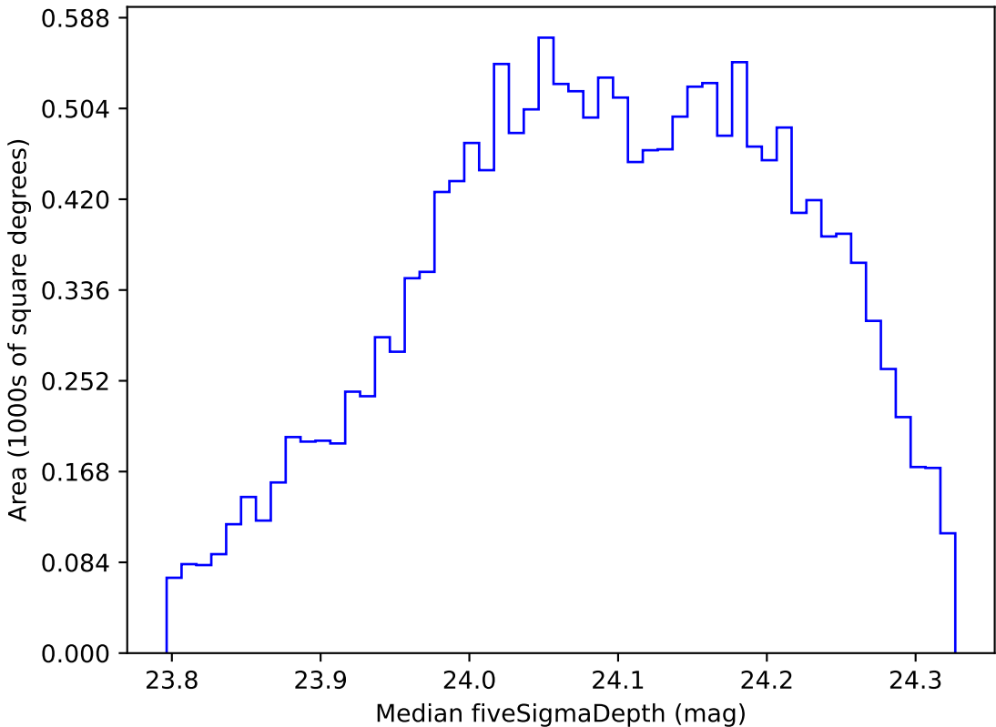
too_ignore_10_1v3.4_10yrs WFD r band: Median fiveSigmaDepth
