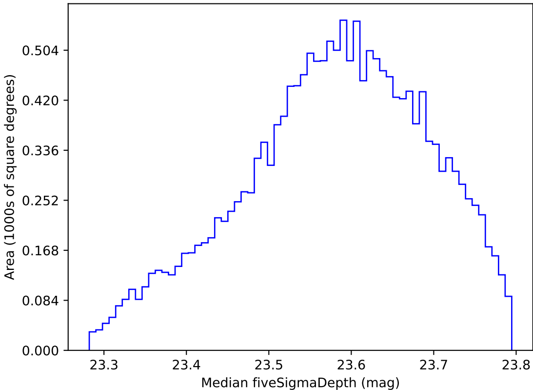
too_ignore_10_1v3.4_10yrs WFD i band: Median fiveSigmaDepth
