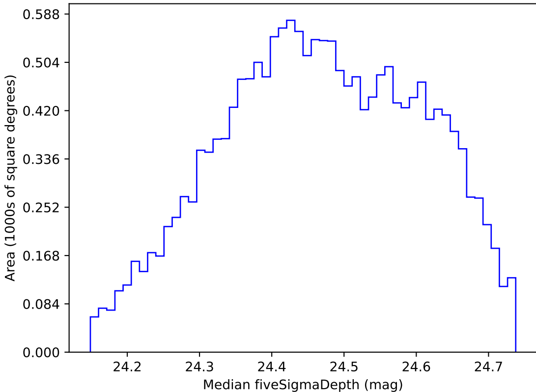
too_ignore_10_1v3.4_10yrs WFD g band: Median fiveSigmaDepth
