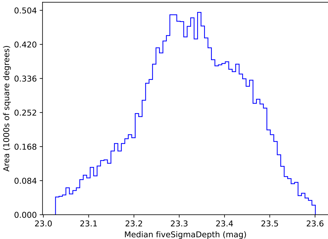
too_ignore_10_1v3.4_10yrs WFD all bands: Median fiveSigmaDepth
