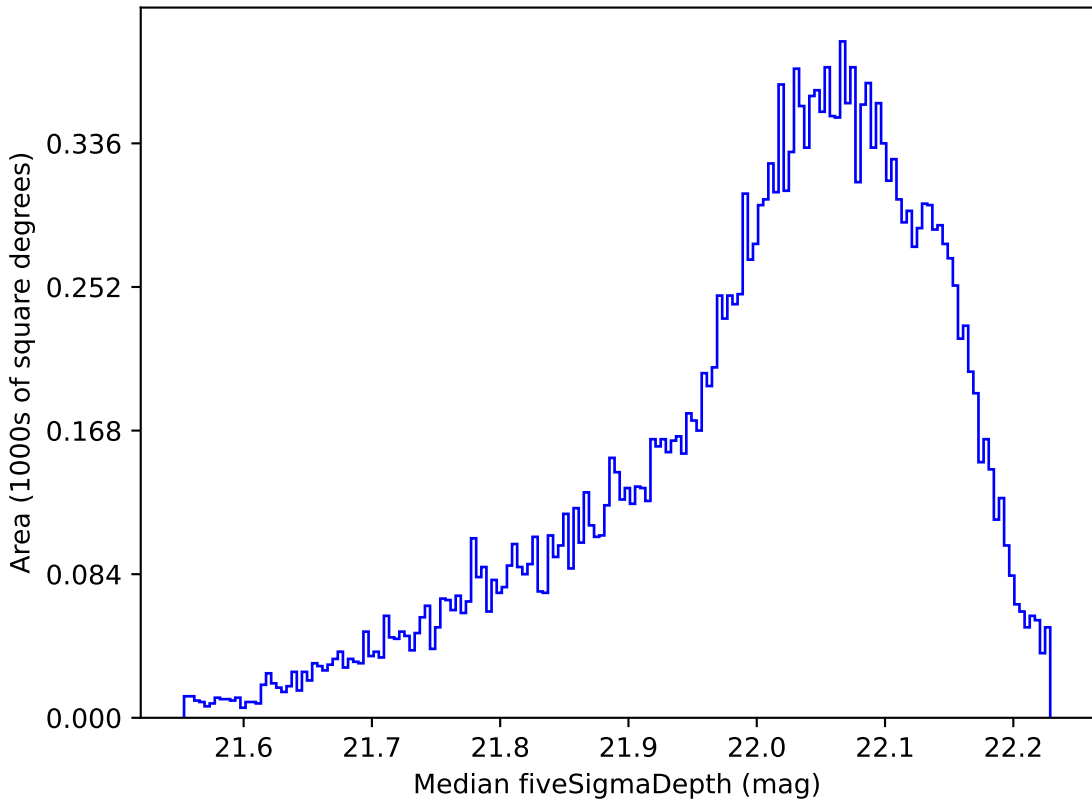
too_ignore_10_1v3.4_10yrs All sky y band: Median fiveSigmaDepth
