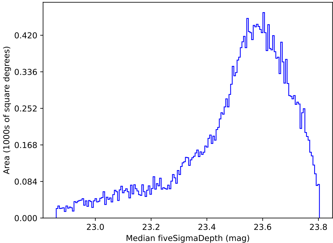
too_ignore_10_1v3.4_10yrs All sky i band: Median fiveSigmaDepth
