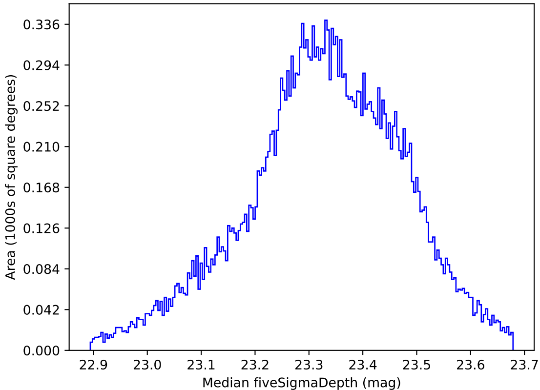
too_ignore_10_1v3.4_10yrs All sky all bands: Median fiveSigmaDepth
