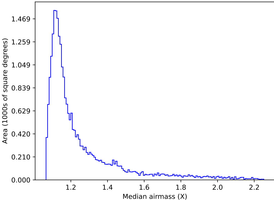
too_ignore_10_1v3.4_10yrs Yr 1 z band: Median airmass
