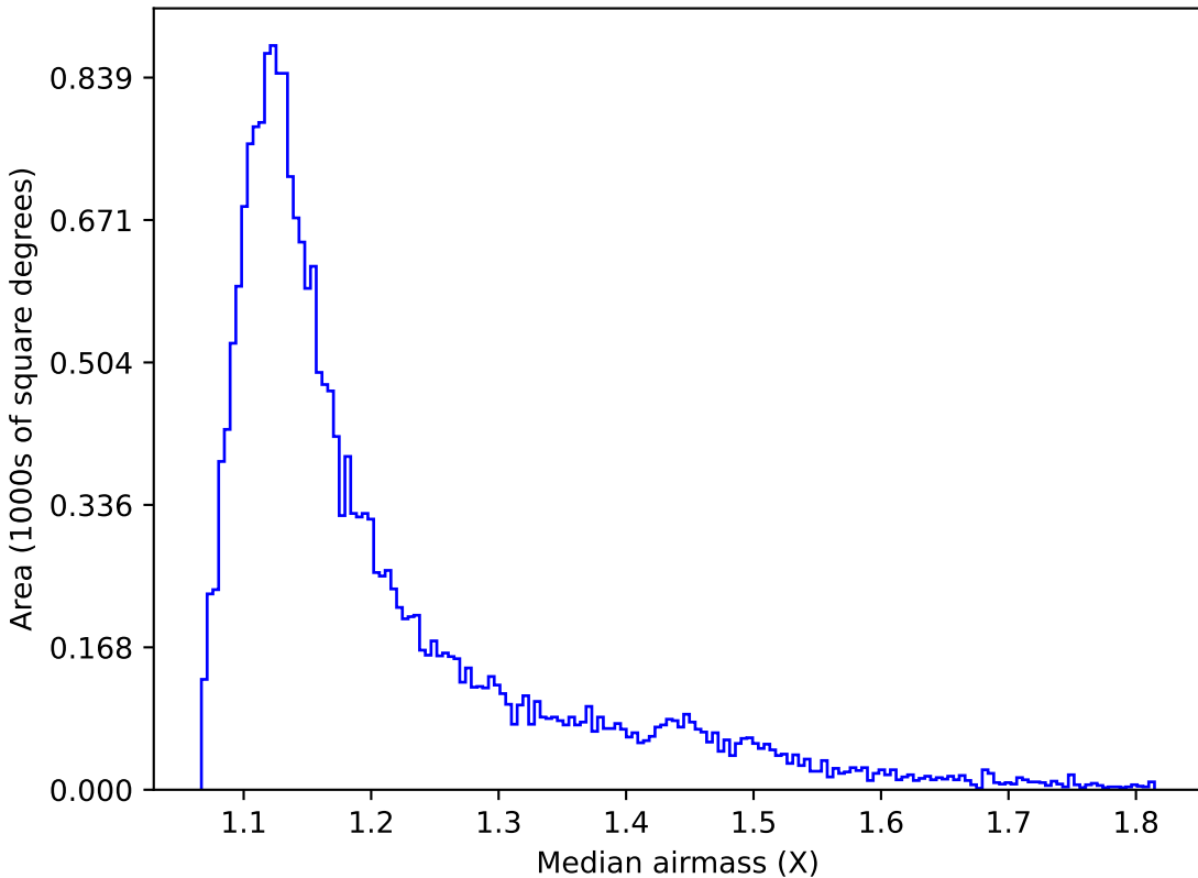
too_ignore_10_1v3.4_10yrs Yr 1 y band: Median airmass
