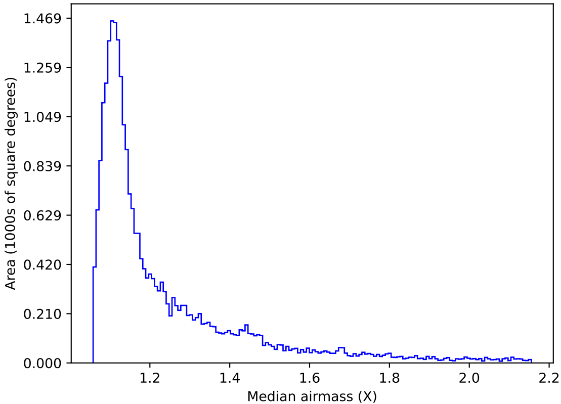
too_ignore_10_1v3.4_10yrs Yr 1 r band: Median airmass
