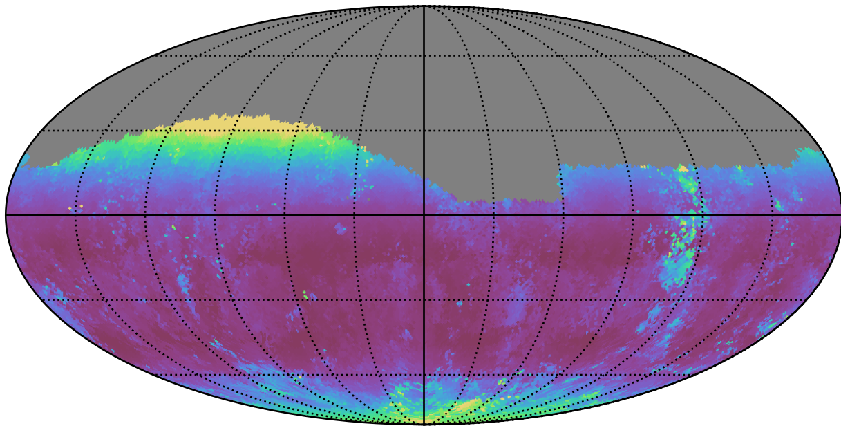
too_ignore_10_1v3.4_10yrs Yr 1 g band: Median airmass
