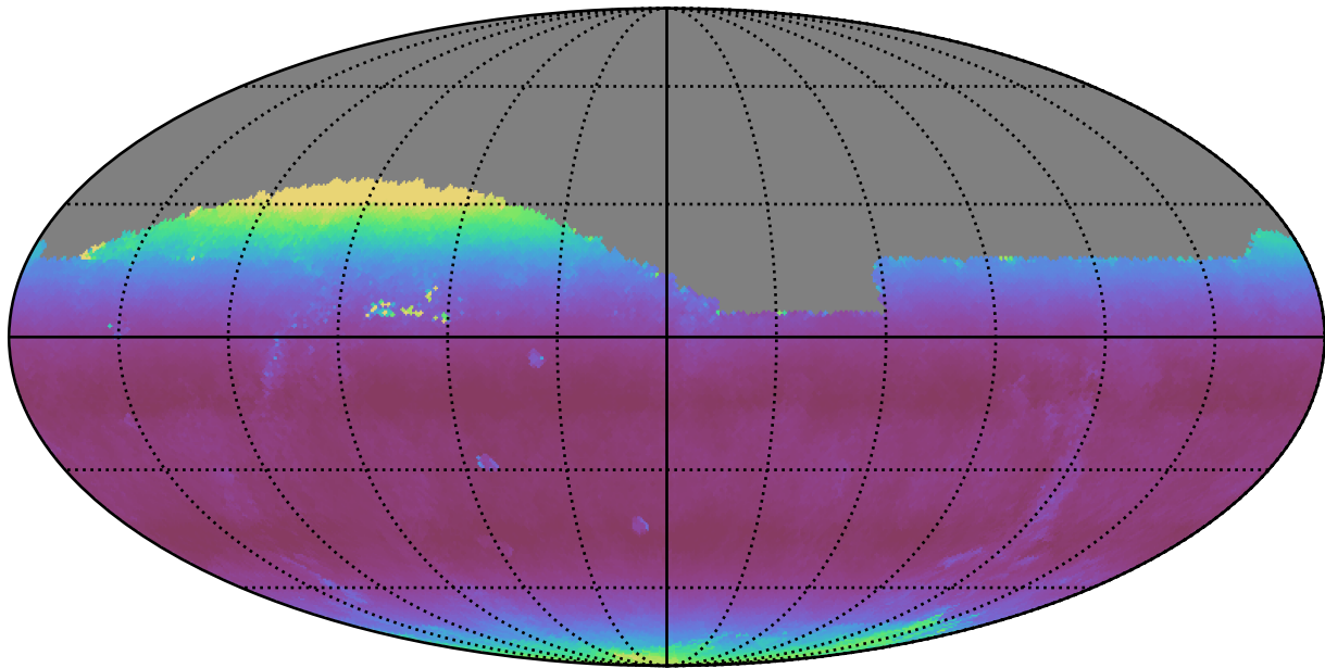
too_ignore_10_1v3.4_10yrs Yr 1 all bands: Median airmass
