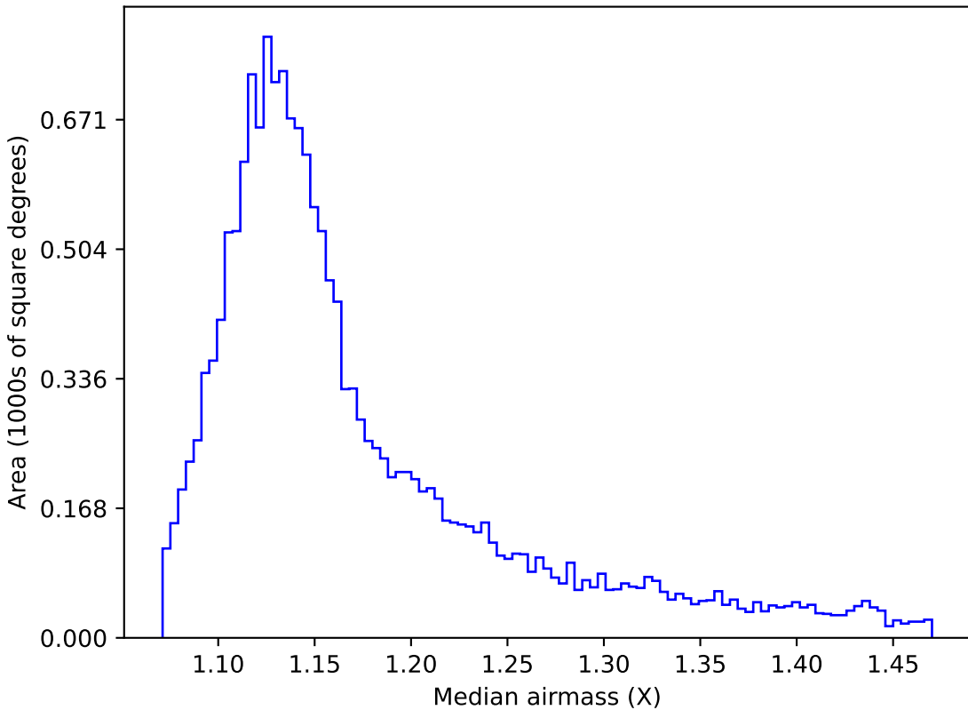
too_ignore_10_1v3.4_10yrs WFD u band: Median airmass
