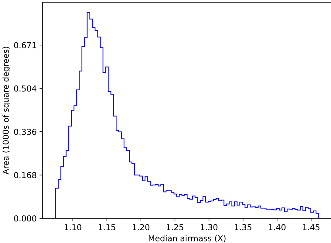
too_ignore_10_1v3.4_10yrs WFD r band: Median airmass
