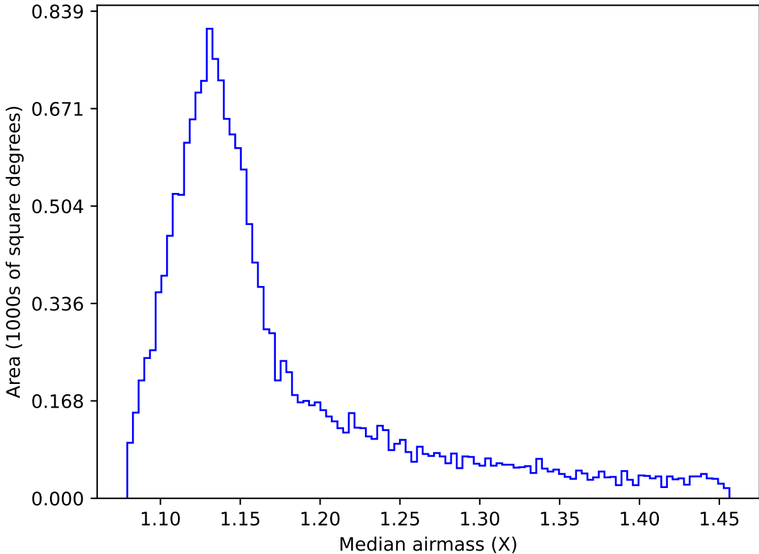
too_ignore_10_1v3.4_10yrs WFD i band: Median airmass
