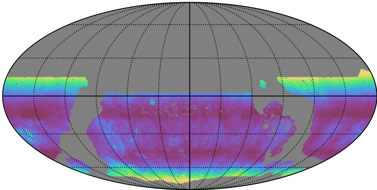
too_ignore_10_1v3.4_10yrs WFD g band: Median airmass
