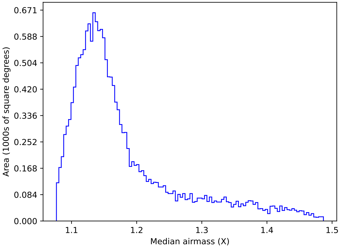
too_ignore_10_1v3.4_10yrs WFD g band: Median airmass
