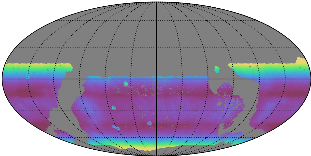
too_ignore_10_1v3.4_10yrs WFD all bands: Median airmass
