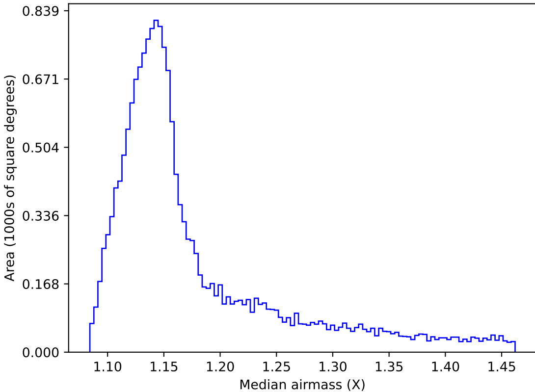
too_ignore_10_1v3.4_10yrs WFD all bands: Median airmass
