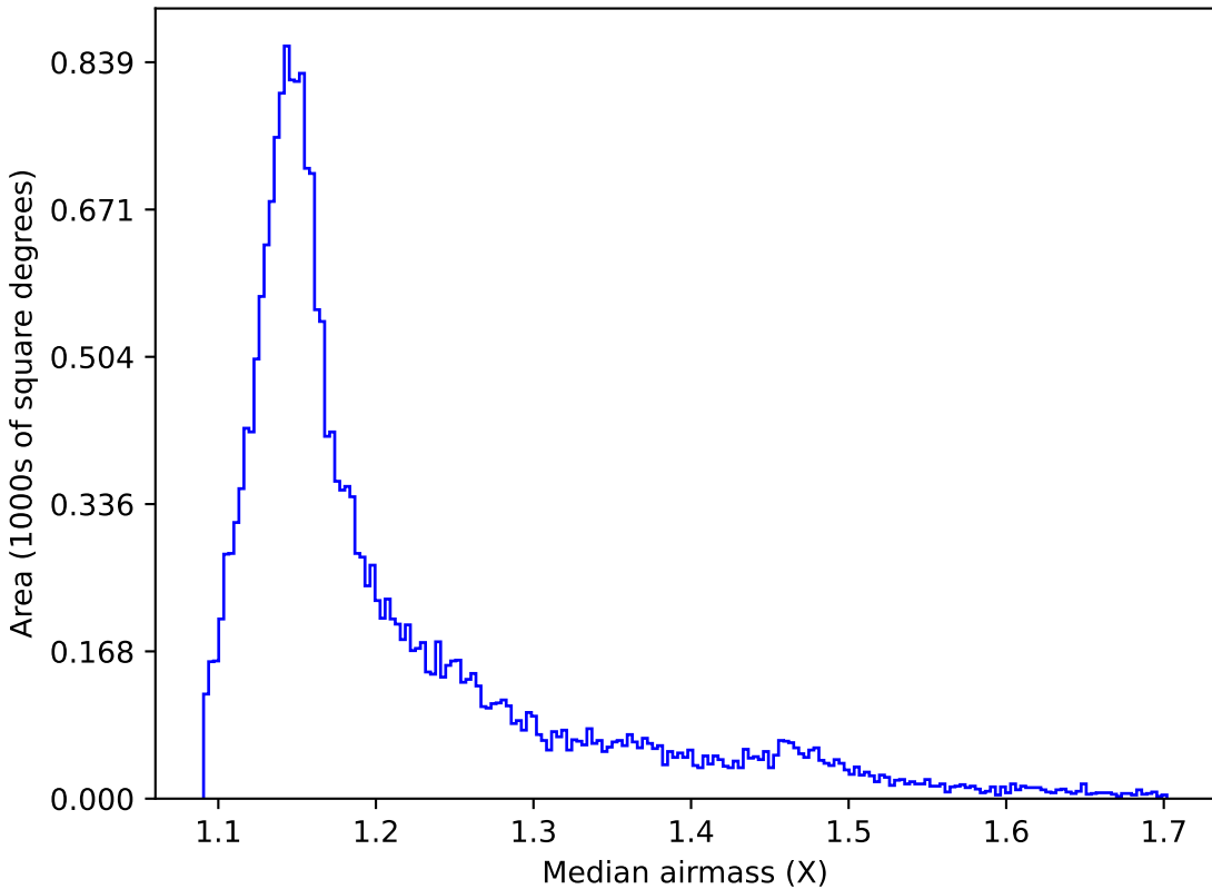
too_ignore_10_1v3.4_10yrs All sky y band: Median airmass
