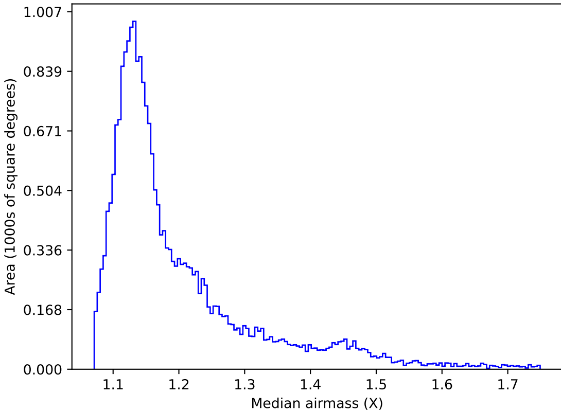
too_ignore_10_1v3.4_10yrs All sky u band: Median airmass
