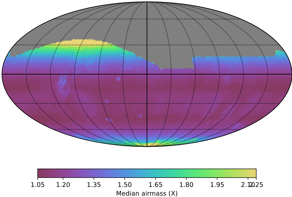
too_ignore_10_1v3.4_10yrs All sky r band: Median airmass
