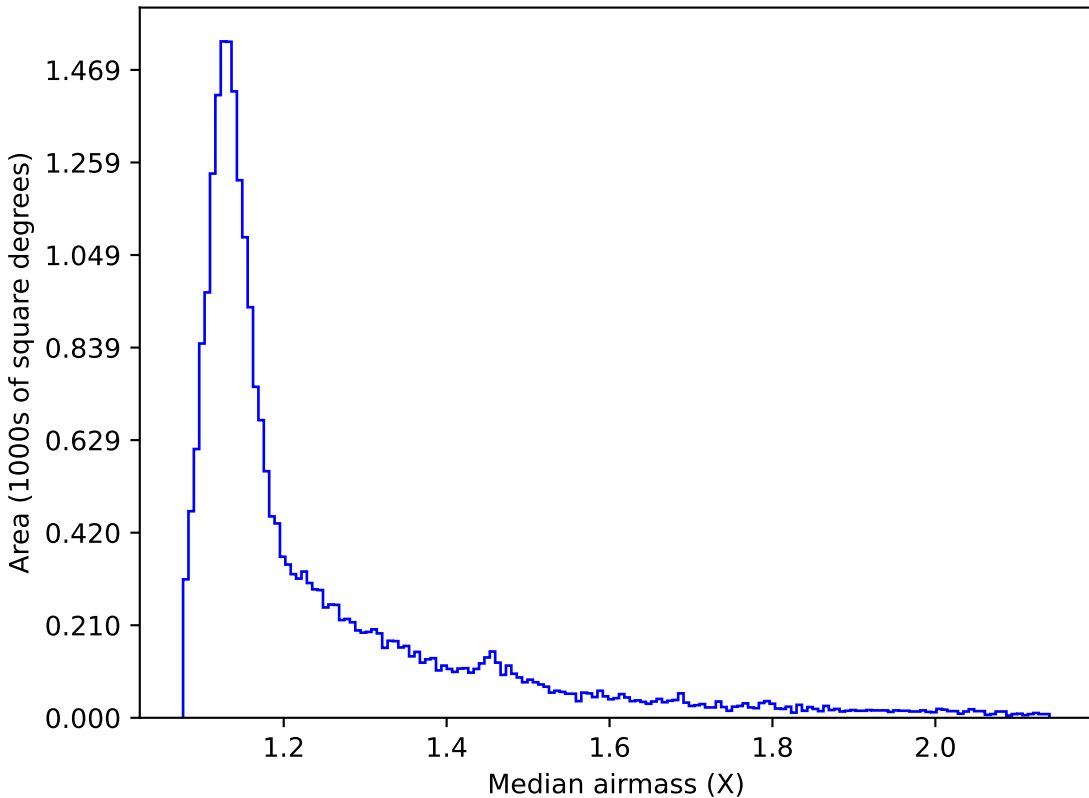
too_ignore_10_1v3.4_10yrs All sky r band: Median airmass
