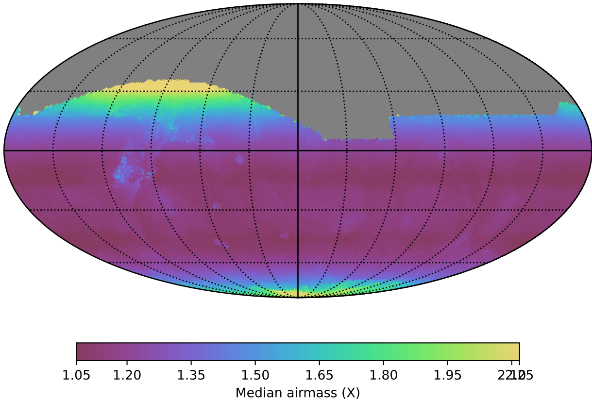
too_ignore_10_1v3.4_10yrs All sky i band: Median airmass
