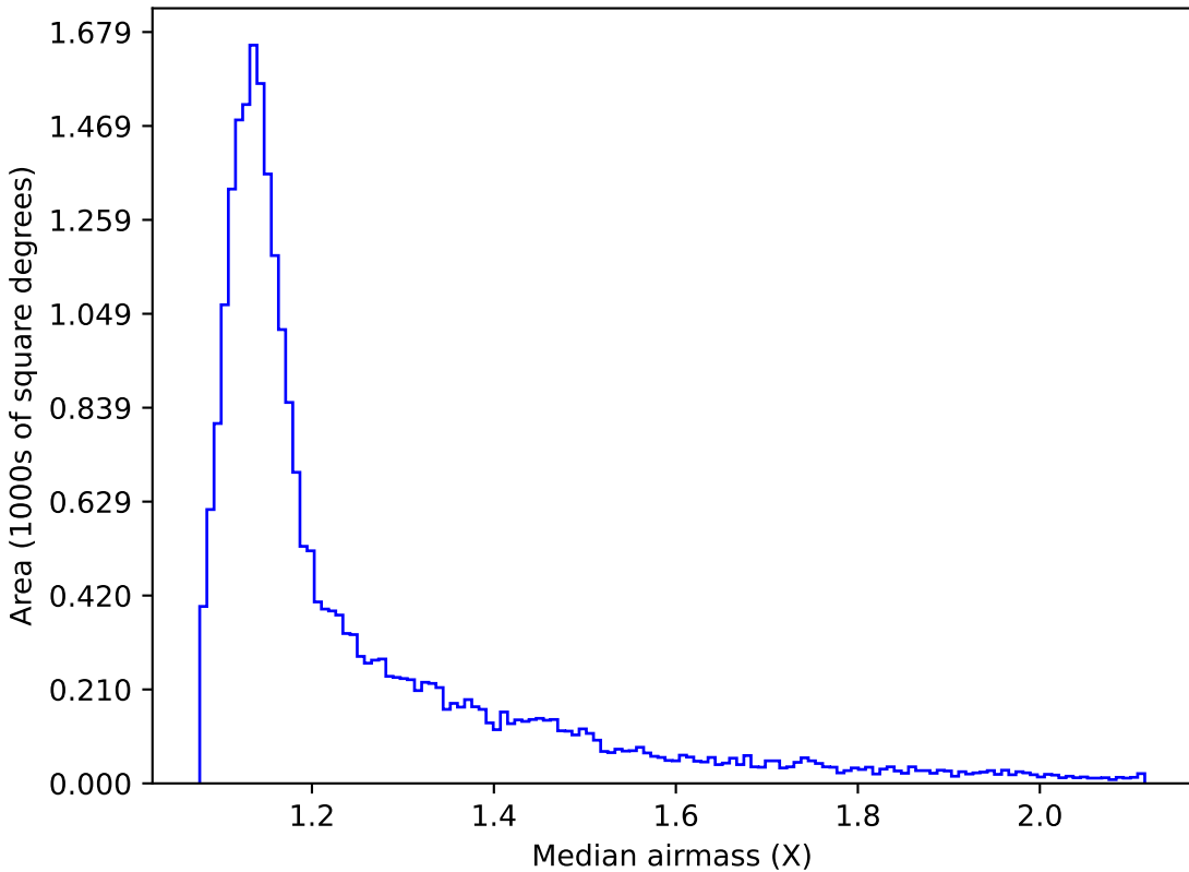
too_ignore_10_1v3.4_10yrs All sky g band: Median airmass
