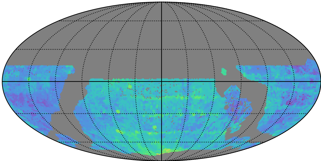
too_ignore_10_1v3.4_10yrs WFD y band: Median Season Length
