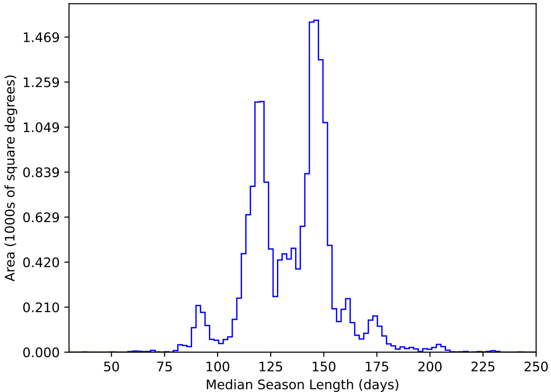
too_ignore_10_1v3.4_10yrs WFD y band: Median Season Length
