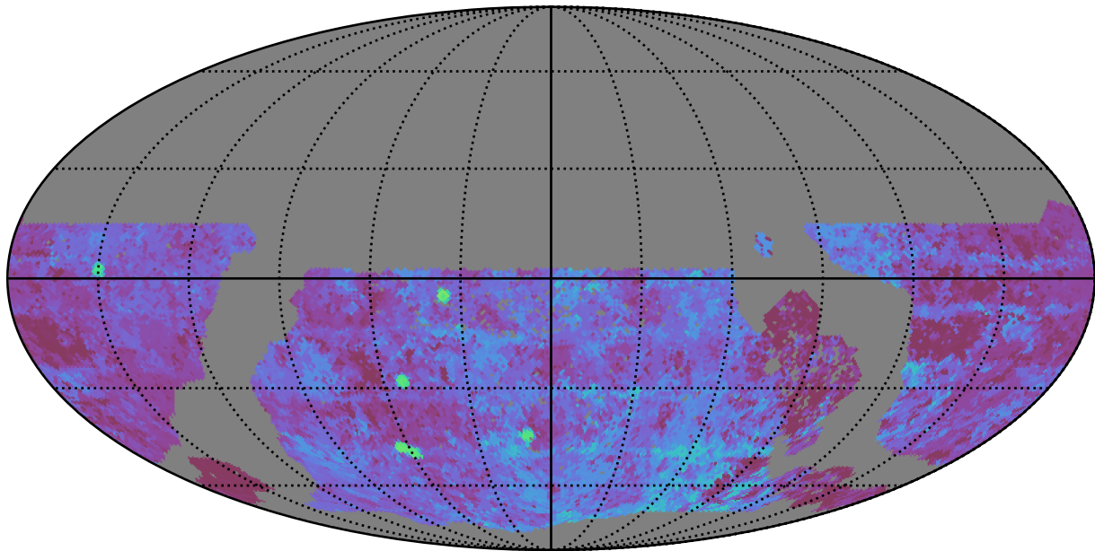
too_ignore_10_1v3.4_10yrs WFD u band: Median Season Length
