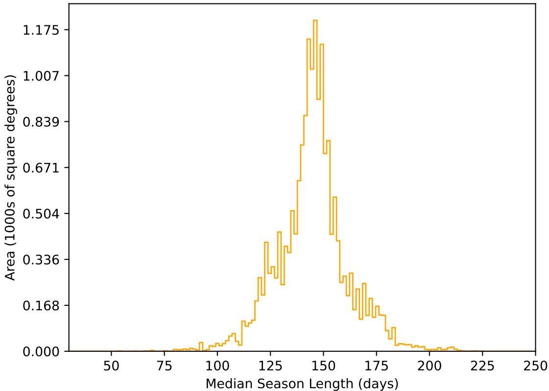
too_ignore_10_1v3.4_10yrs WFD r band: Median Season Length
