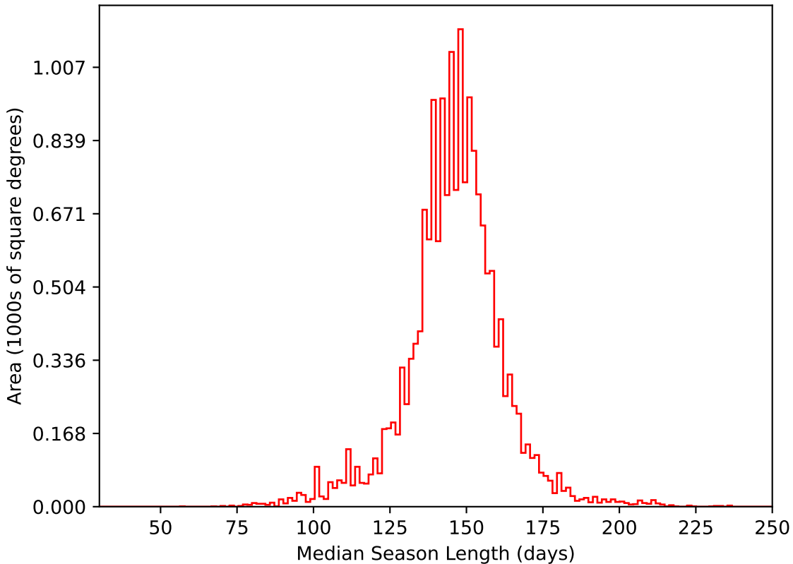
too_ignore_10_1v3.4_10yrs WFD i band: Median Season Length
