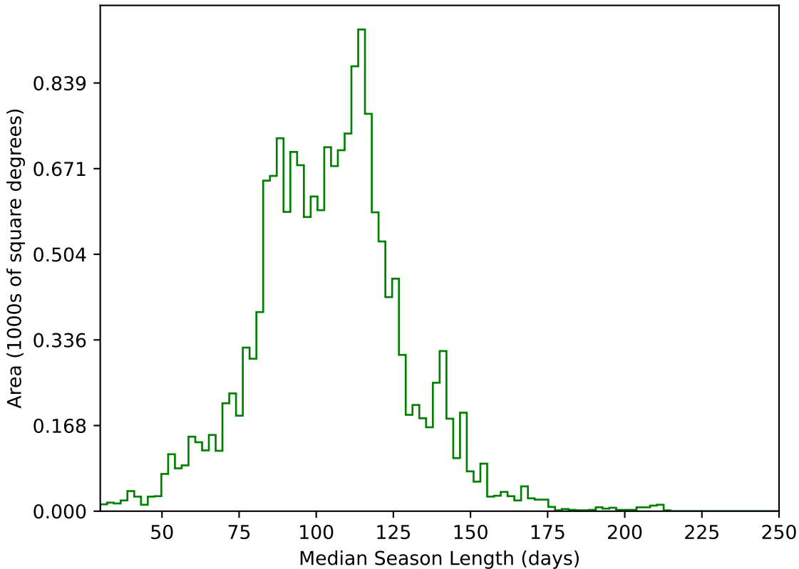
too_ignore_10_1v3.4_10yrs WFD g band: Median Season Length
