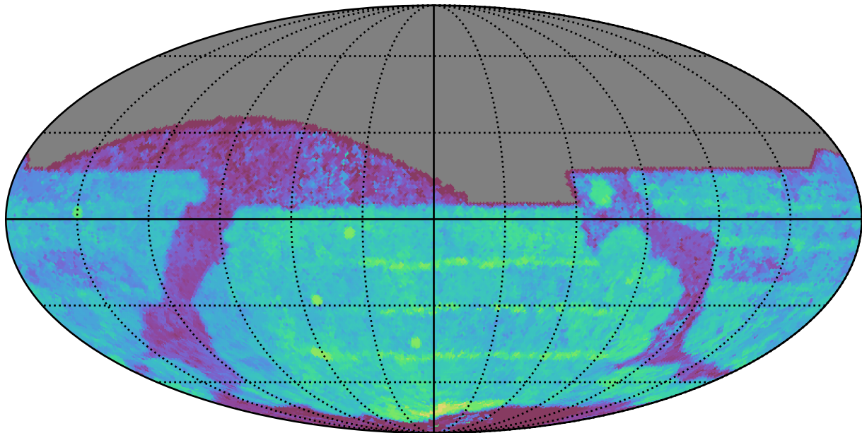
too_ignore_10_1v3.4_10yrs All sky z band: Median Season Length
