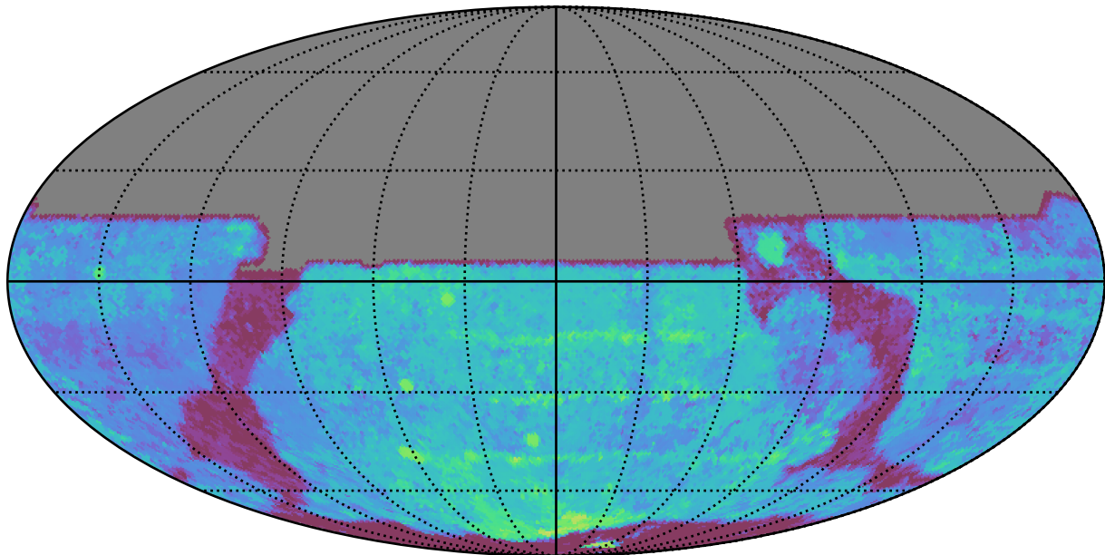
too_ignore_10_1v3.4_10yrs All sky y band: Median Season Length
