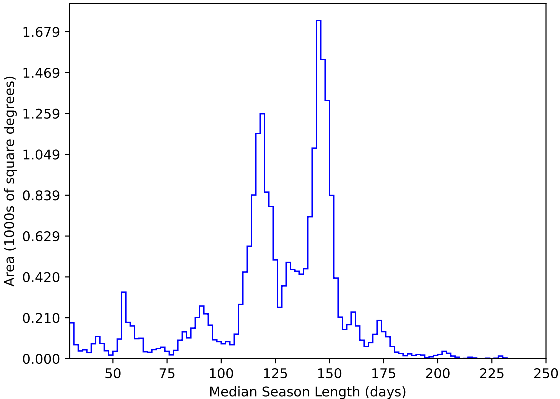
too_ignore_10_1v3.4_10yrs All sky y band: Median Season Length
