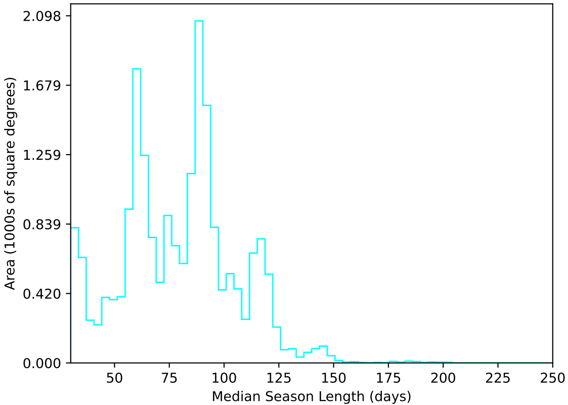
too_ignore_10_1v3.4_10yrs All sky u band: Median Season Length
