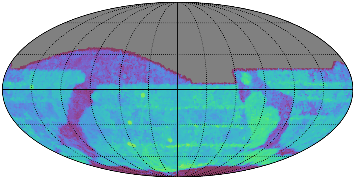
too_ignore_10_1v3.4_10yrs All sky r band: Median Season Length
