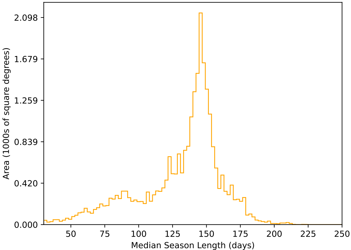
too_ignore_10_1v3.4_10yrs All sky r band: Median Season Length
