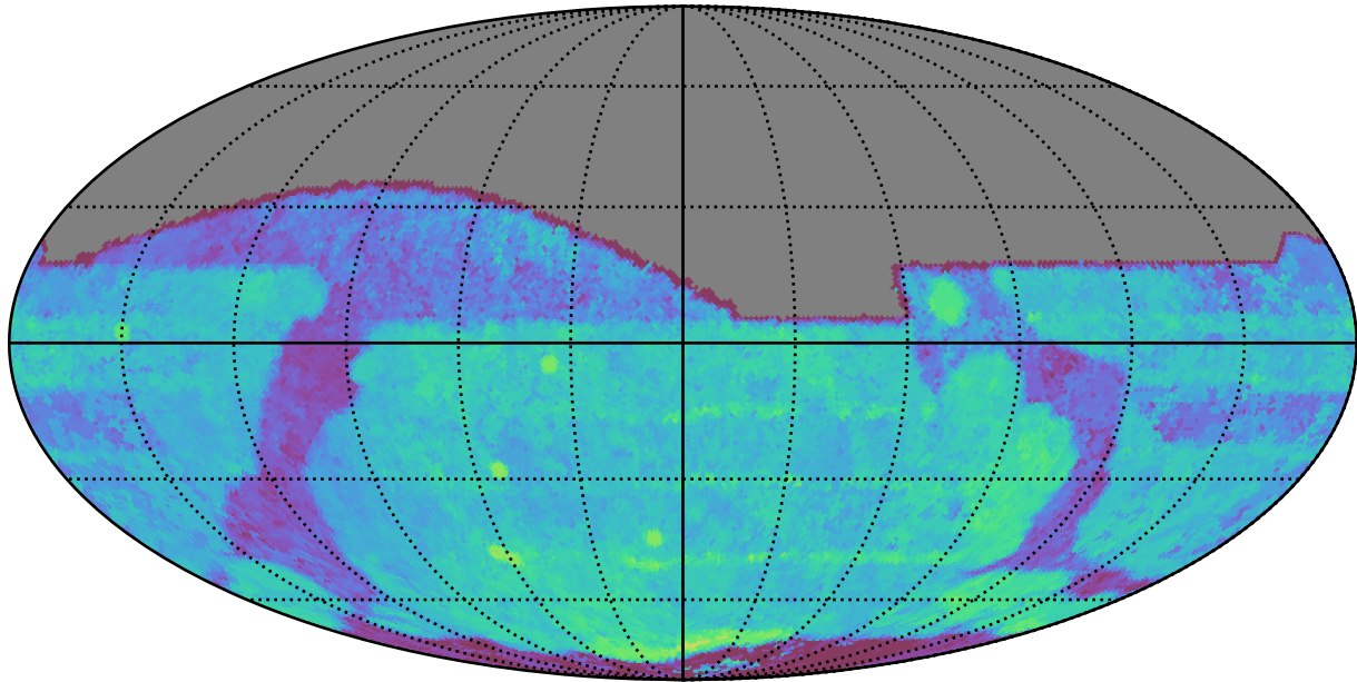
too_ignore_10_1v3.4_10yrs All sky i band: Median Season Length
