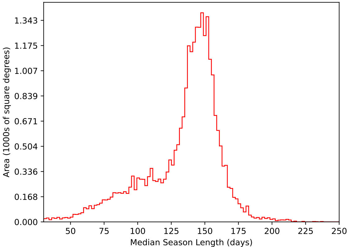
too_ignore_10_1v3.4_10yrs All sky i band: Median Season Length
