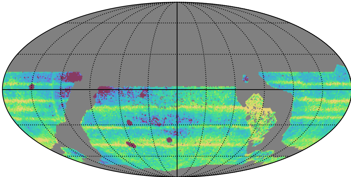
too_ignore_10_1v3.4_10yrs WFD: Median Intra-Night Gap
