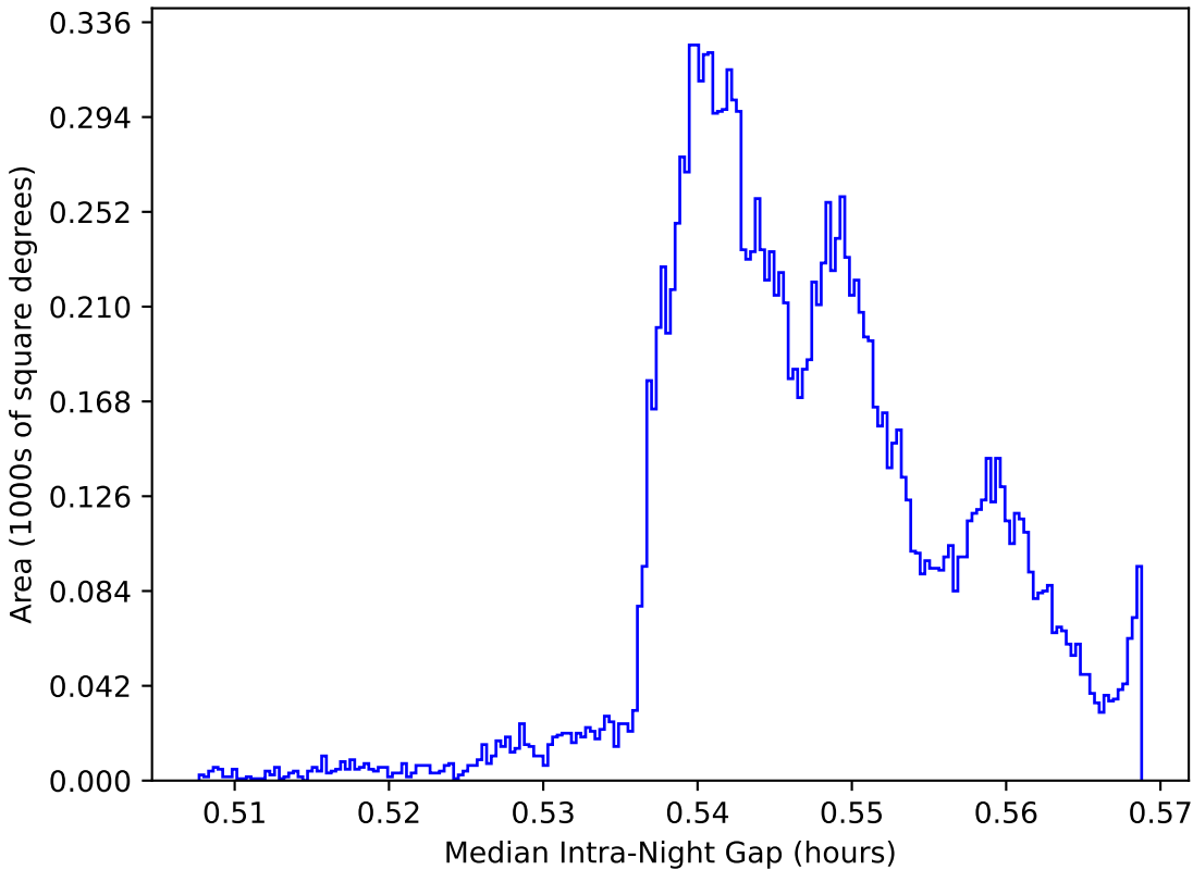
too_ignore_10_1v3.4_10yrs WFD: Median Intra-Night Gap
