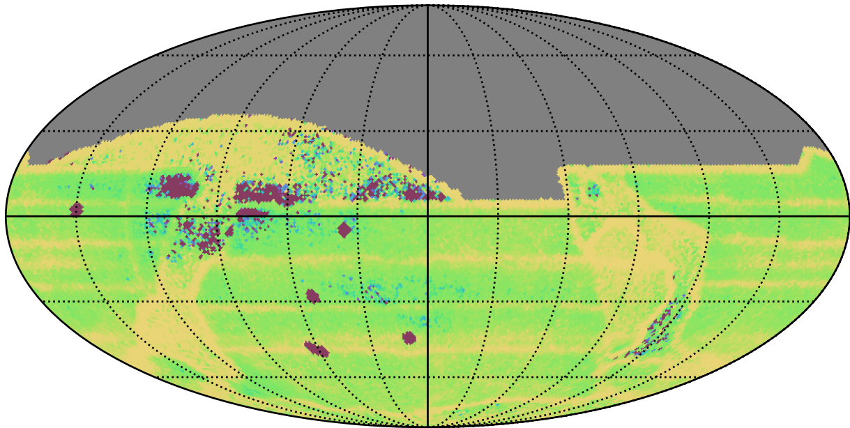
too_ignore_10_1v3.4_10yrs All sky: Median Intra-Night Gap
